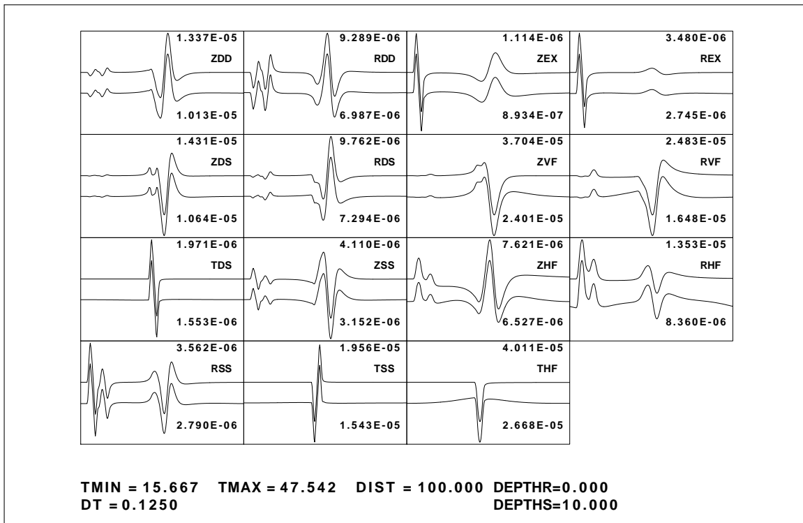
Fig. 3b. Comparison of the initial ground velocity (top trace) to the reconstructed ground velocity (bottom trace).
